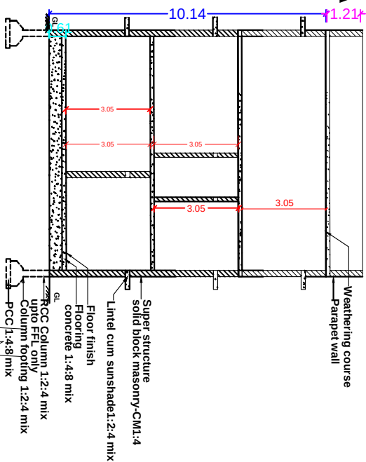
SECTION ELEVATION
