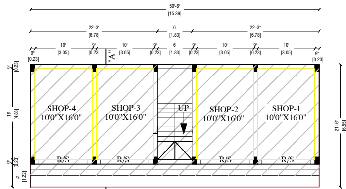
EXIST. GROUND FLOOR PLAN
