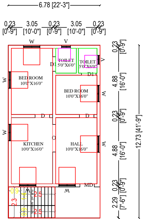
PROPOSED PLAN
