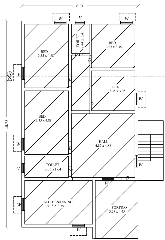
FLOOR PLAN
