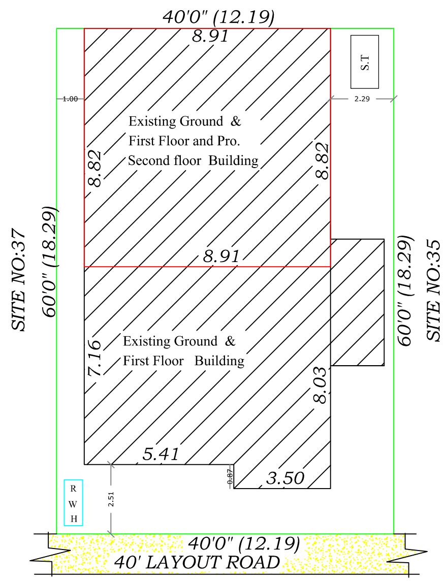
SITE PLAN
