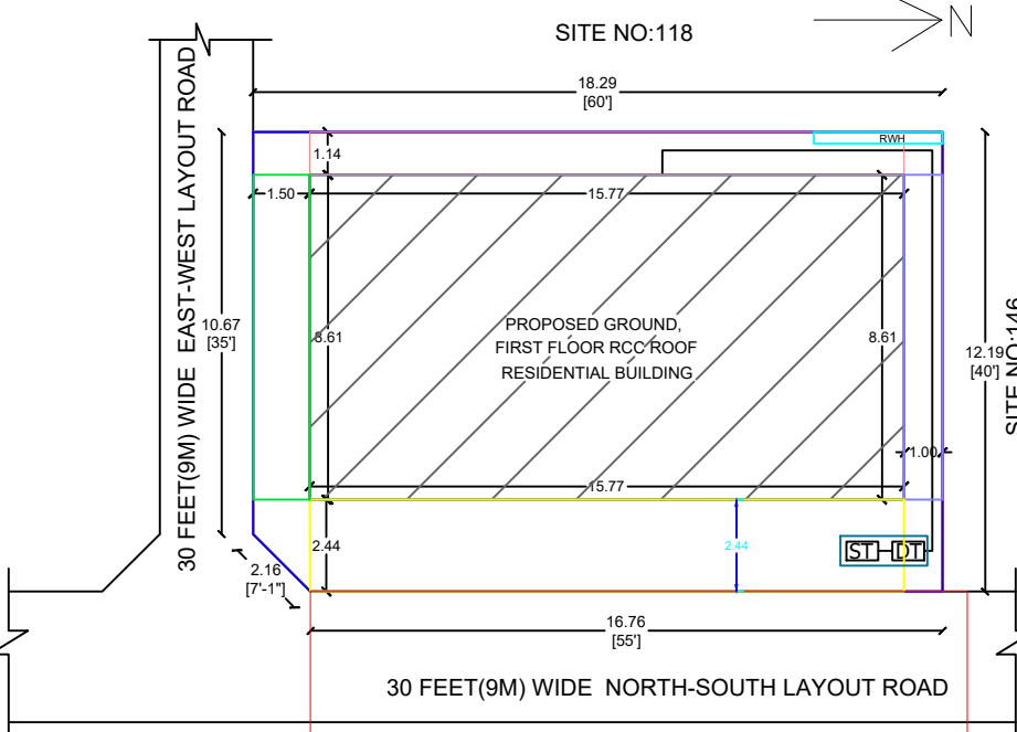
SITE PLAN
