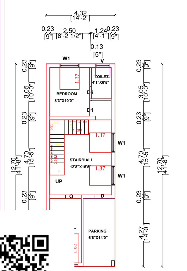
1 Floor Plan
