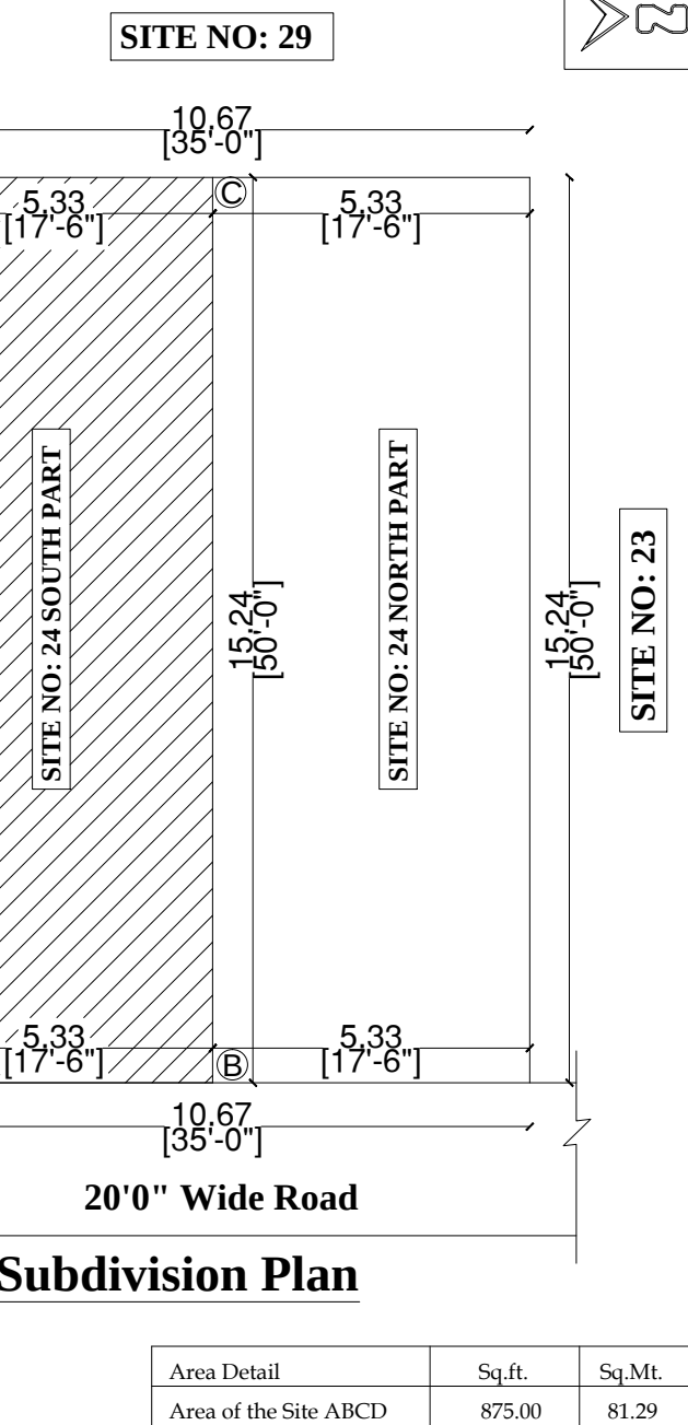
Site Plan
