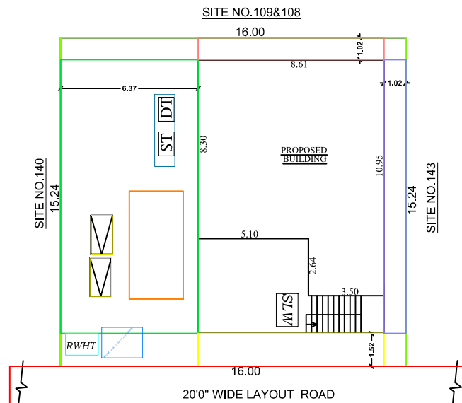
SITE PLAN
