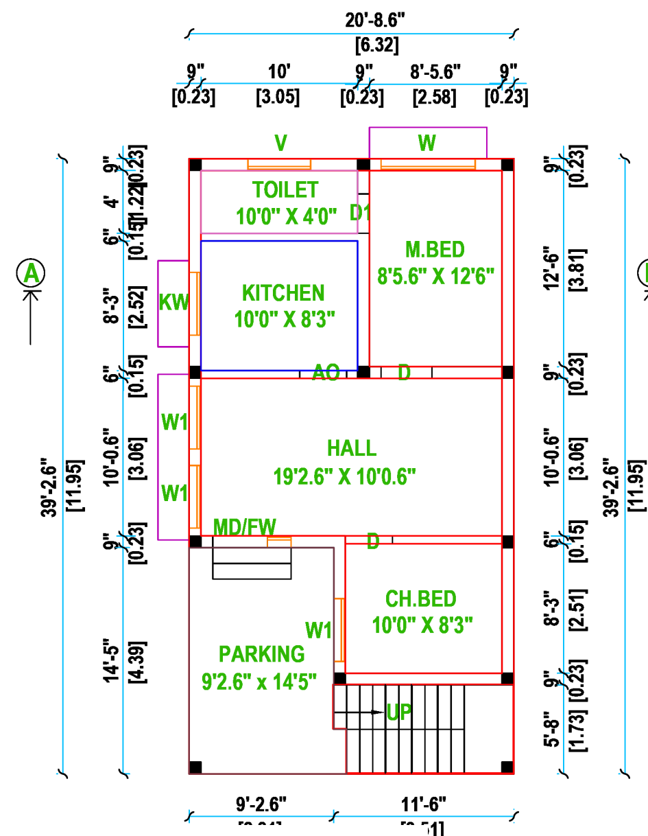
FLOOR PLAN
