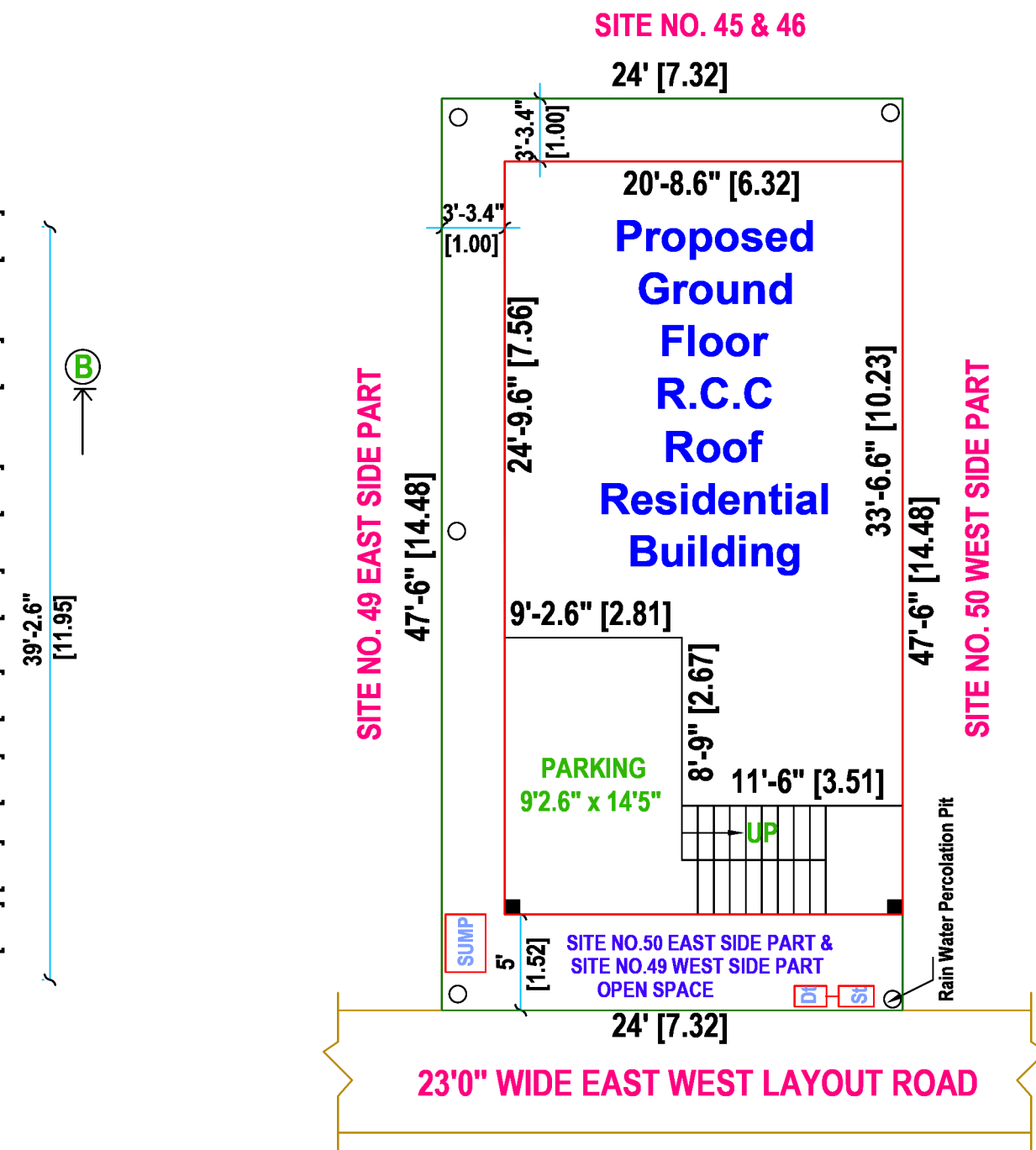
SITE PLAN (SCALE - 1" : 8' 0")
