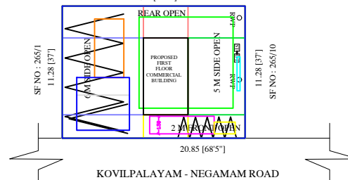
PROPOSED FIRST FLOOR PLAN
