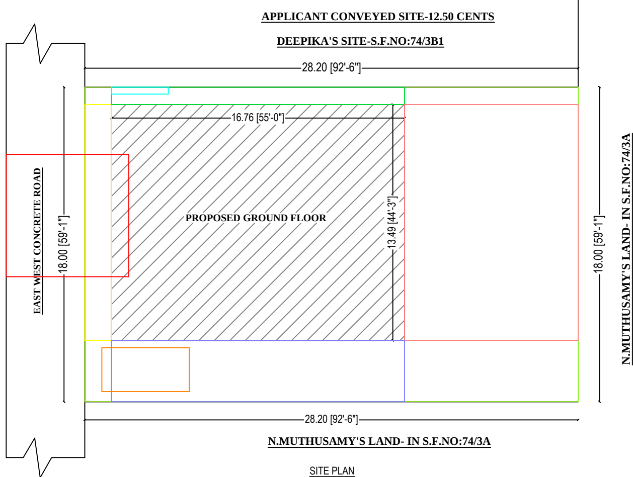
SITE PLAN
