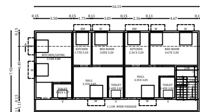
PROPOSED FIRST FLOOR
