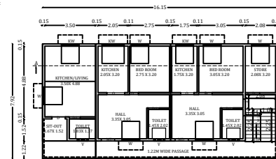
PRO.ADDL.G.FLOOR PLAN
