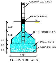
COLUMN DETAILS
