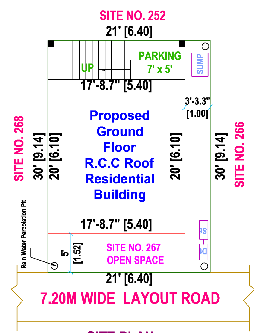
SITE PLAN (SCALE - 1" : 8' 0")
