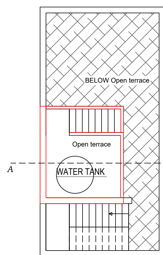
PROPOSED TERRACE FLOOR
