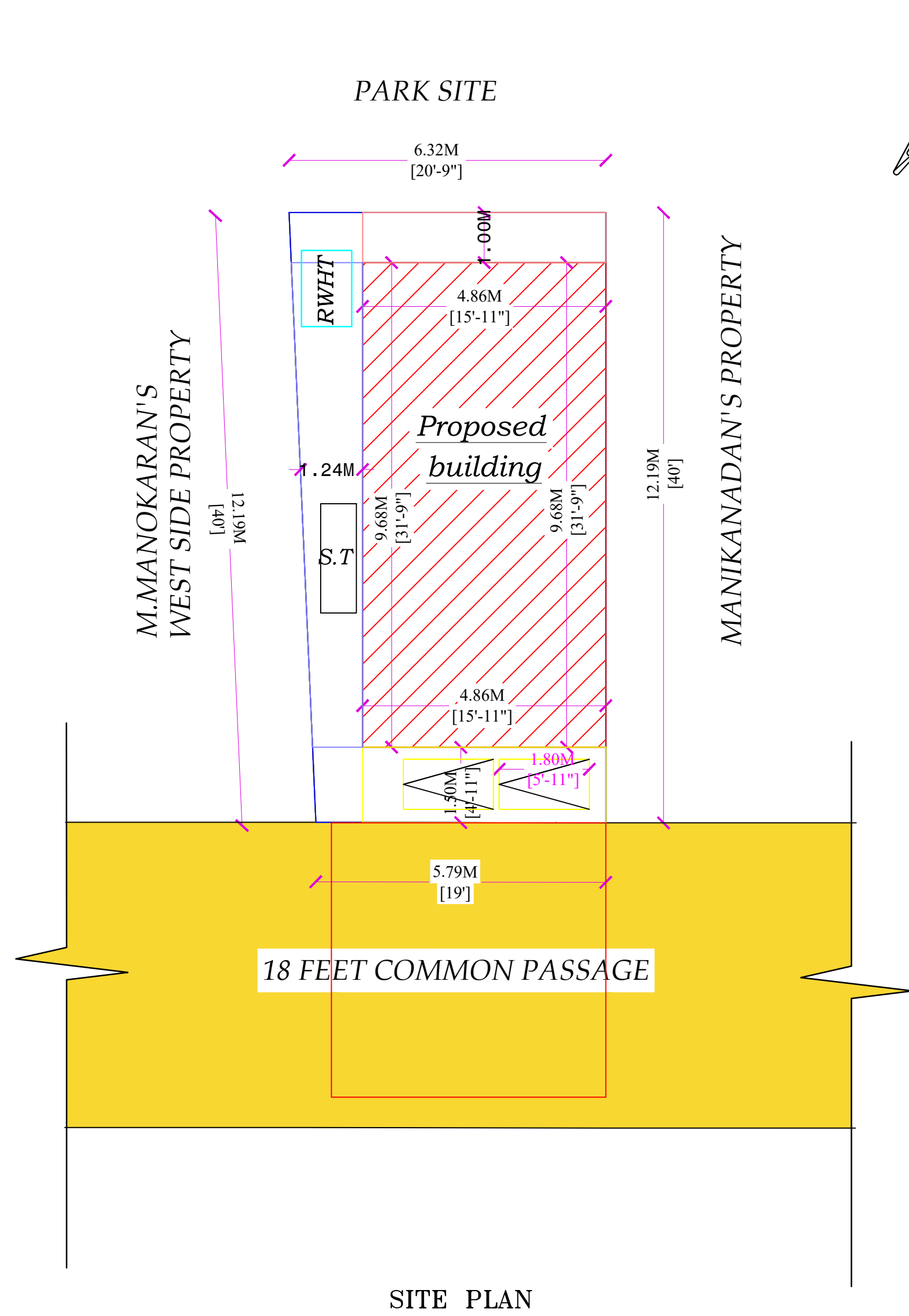
SITE PLAN
