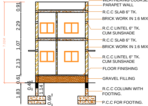
CROSS SECTION AT A-A
