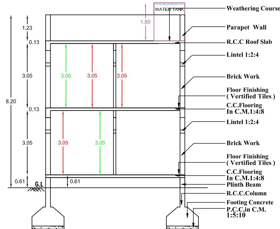
CROSS SECTION A-A
