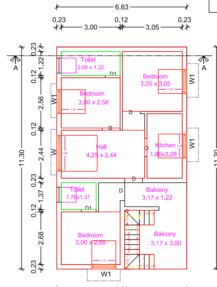
PRO.ADDITIONAL FIRST FLOOR PLAN
