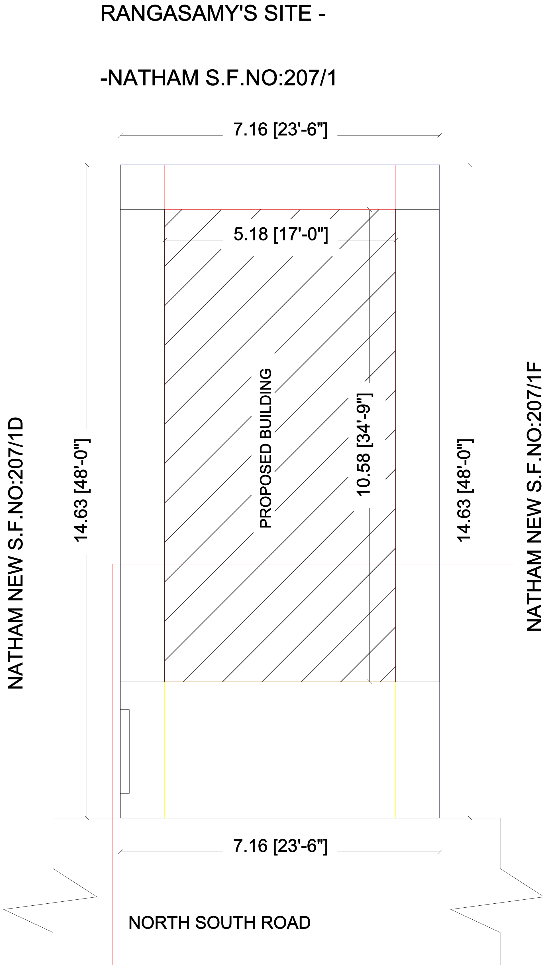
SITE PLAN
