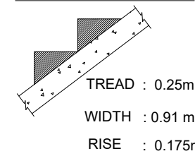
STAIRCASE DETAIL:
