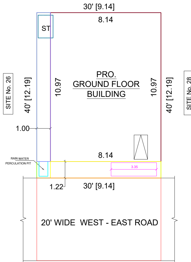
SITE PLAN
