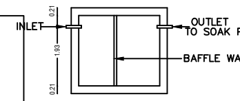
PLAN SEPTIC. TANK
