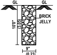
PERCULATION PIT
