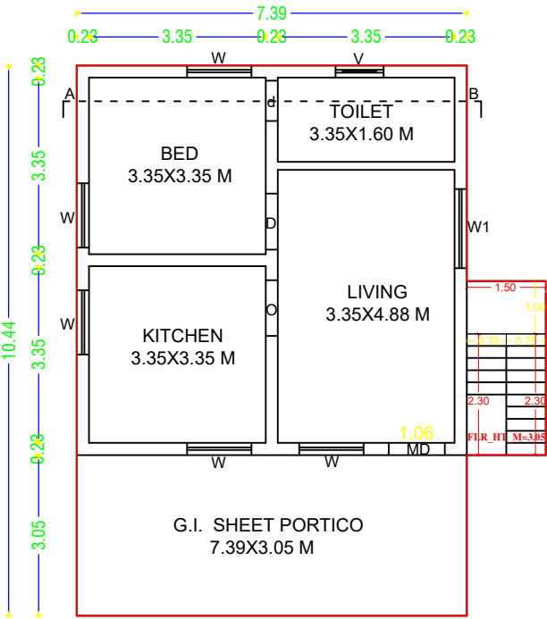
EXG. GROUND FLOOR PLAN
