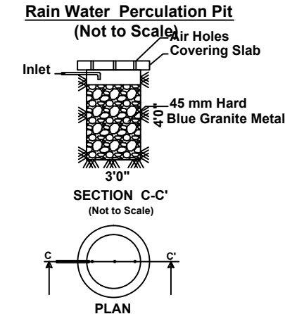
Rain Water Perculation Pit (Not to Scale)
