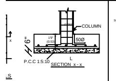
COMPOUND WALL DETAIL
