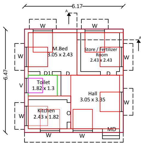
PRO.GF PLAN
