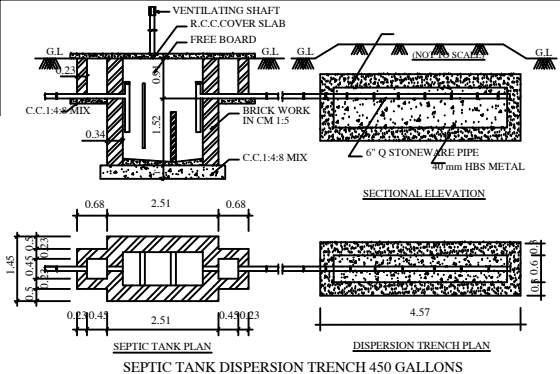
SEPTIC TANK DISPERSION TRENCH 450 GALLONS
