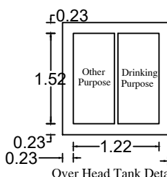
Over Head Tank Details
