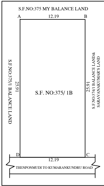
LOCATION PLAN
