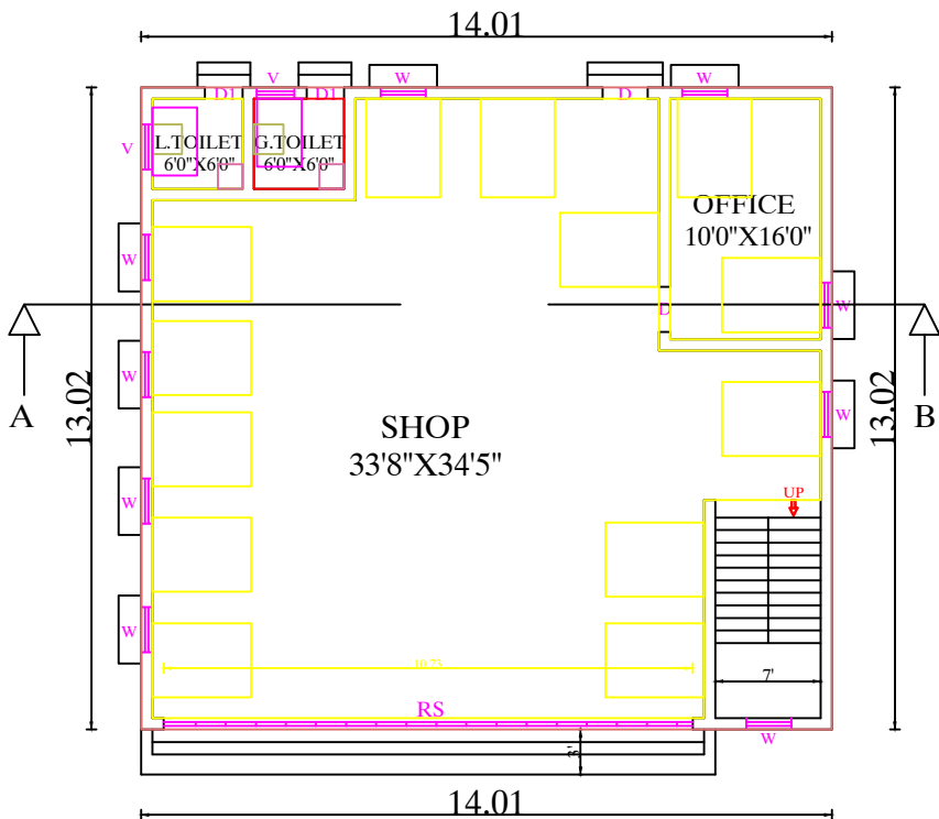
PROPOSED GROUND FLOOR
