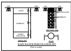
RAIN WATER PERCOLATION PIT
