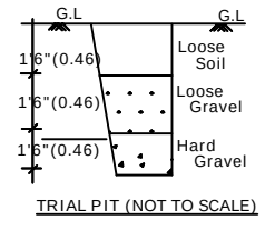
TRIAL PIT (NOT TO SCALE)
