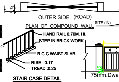
STAIR CASE DETAIL
