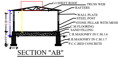
SECTION "AB"
