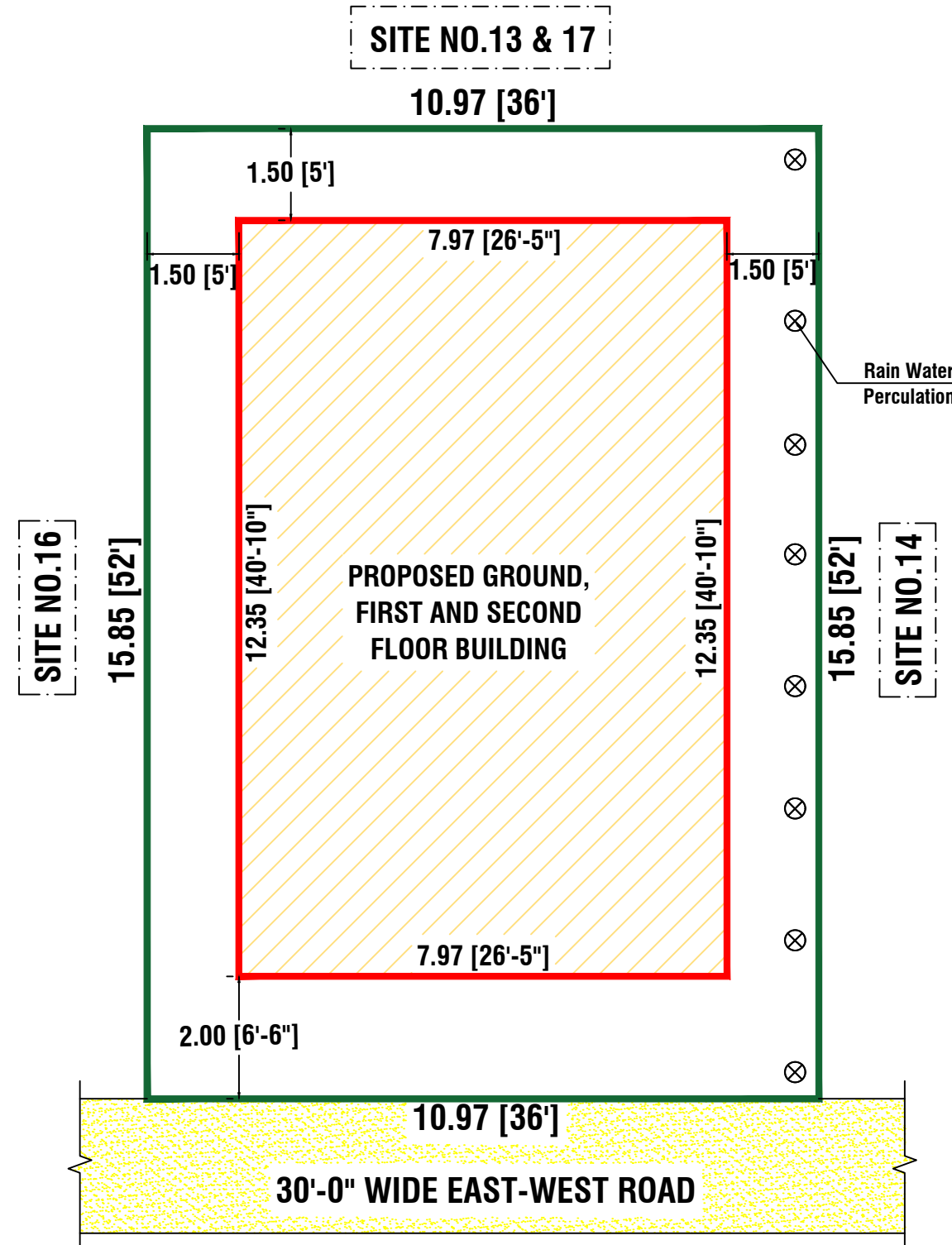
SITE PLAN
