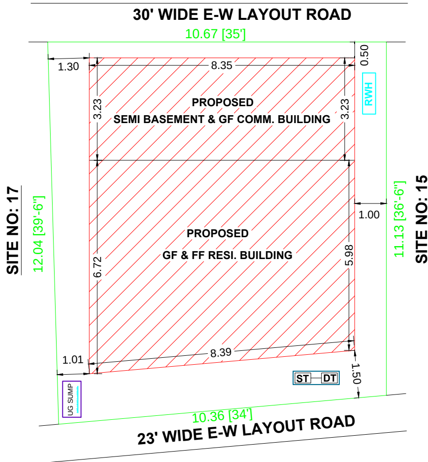
SITE PLAN
