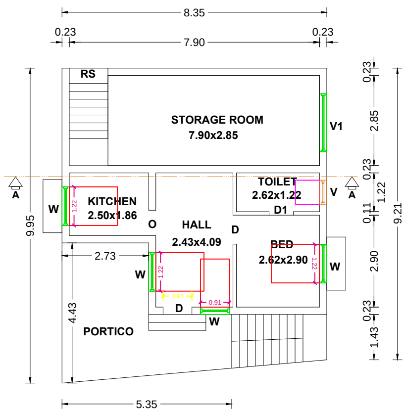
SEMI BASEMENT & GROUND FLOOR PLAN
