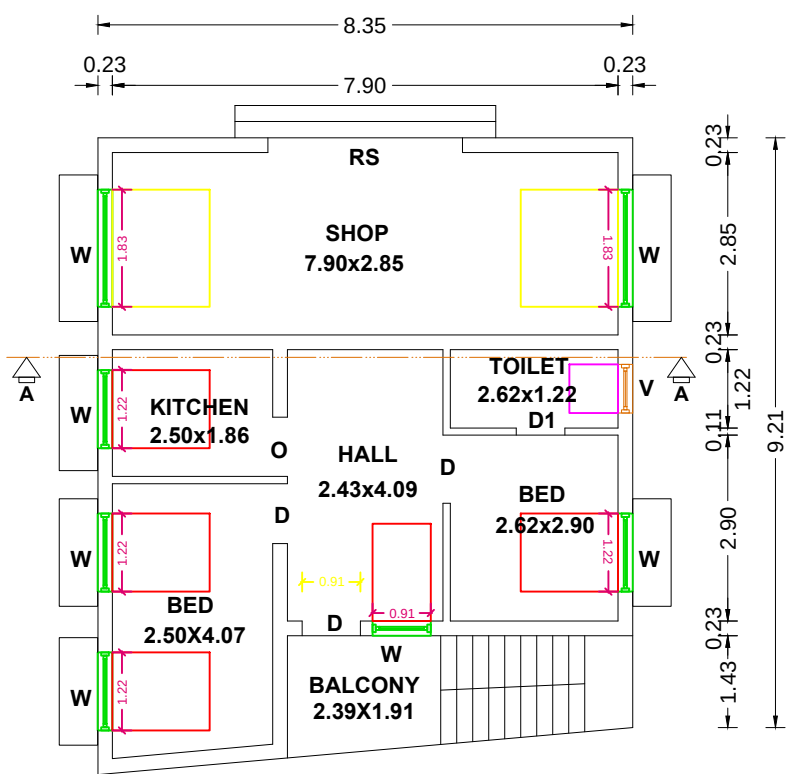
GROUND & FIRST FLOOR PLAN
