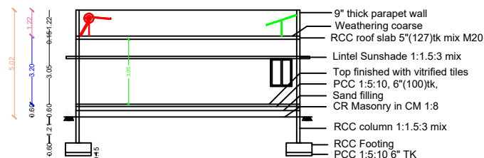
SECTION ON "AA"
