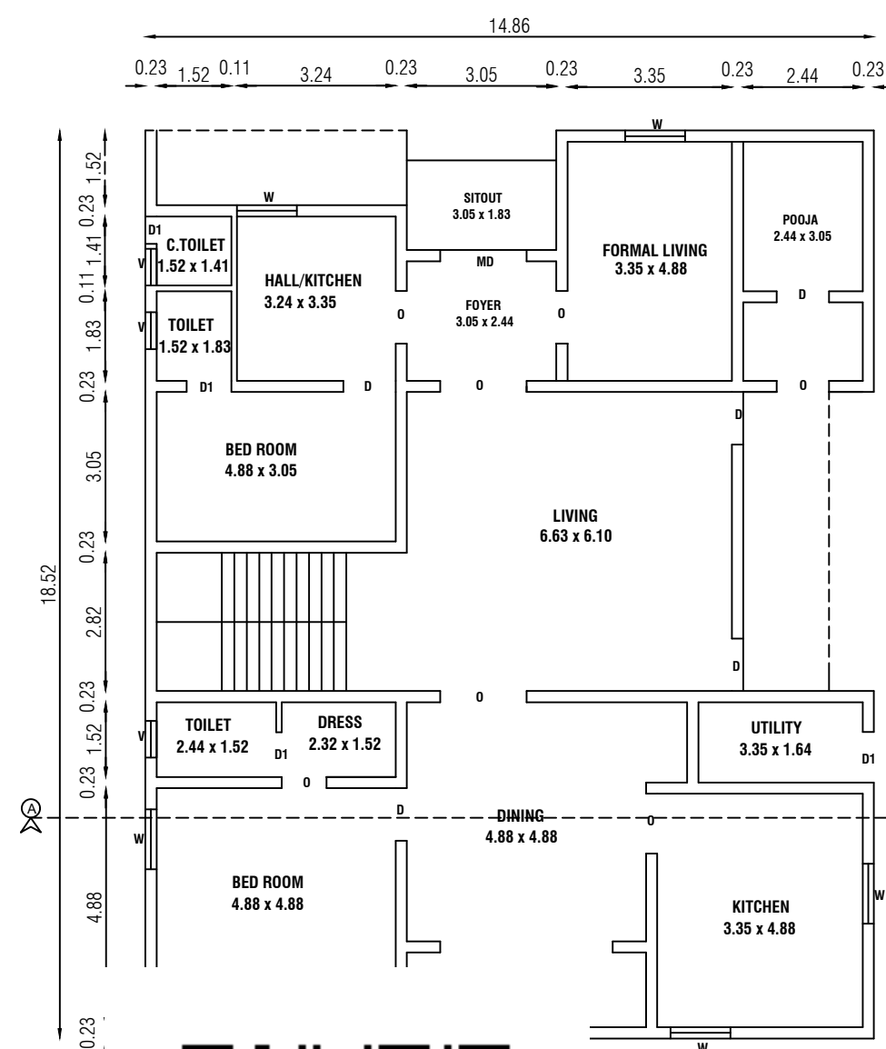
PLAN
