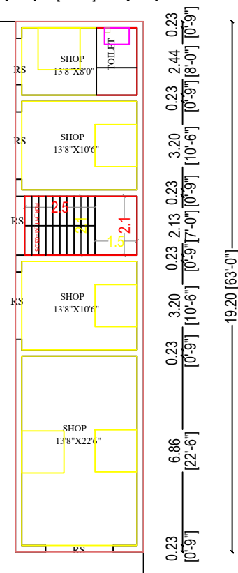
PROPOSED FIRST FLOOR PLAN
