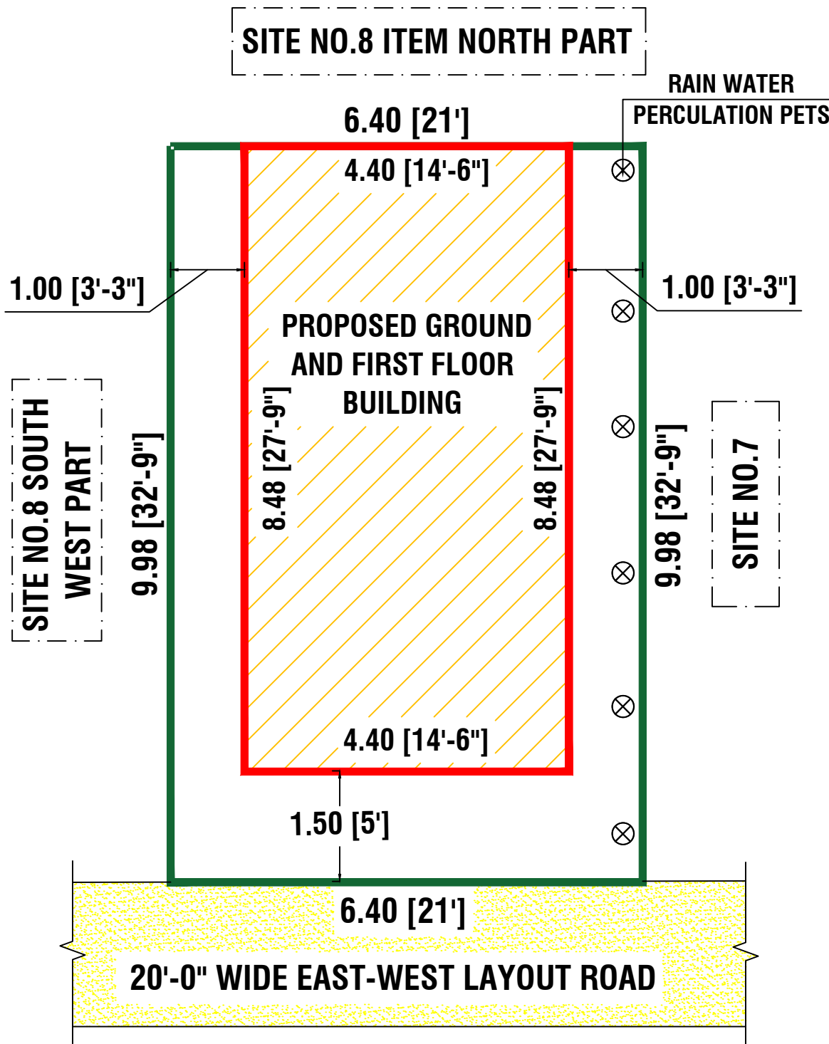
SITE PLAN
