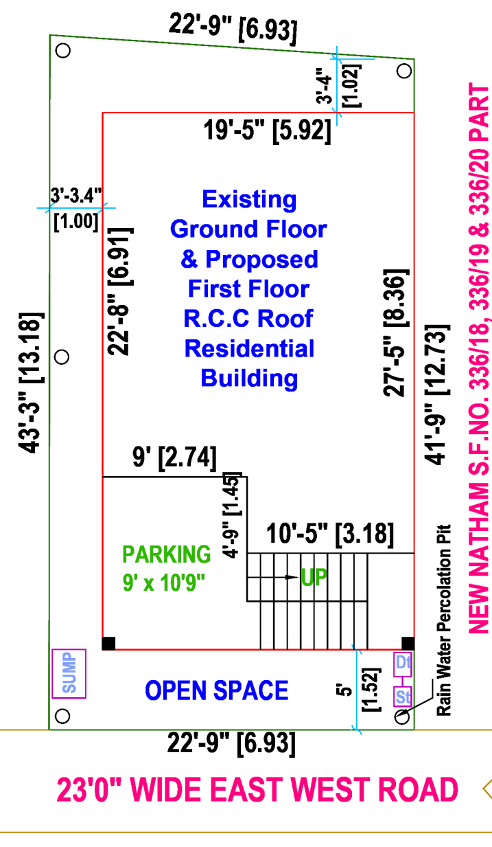
SITE PLAN (SCALE - 1" : 8' 0")
