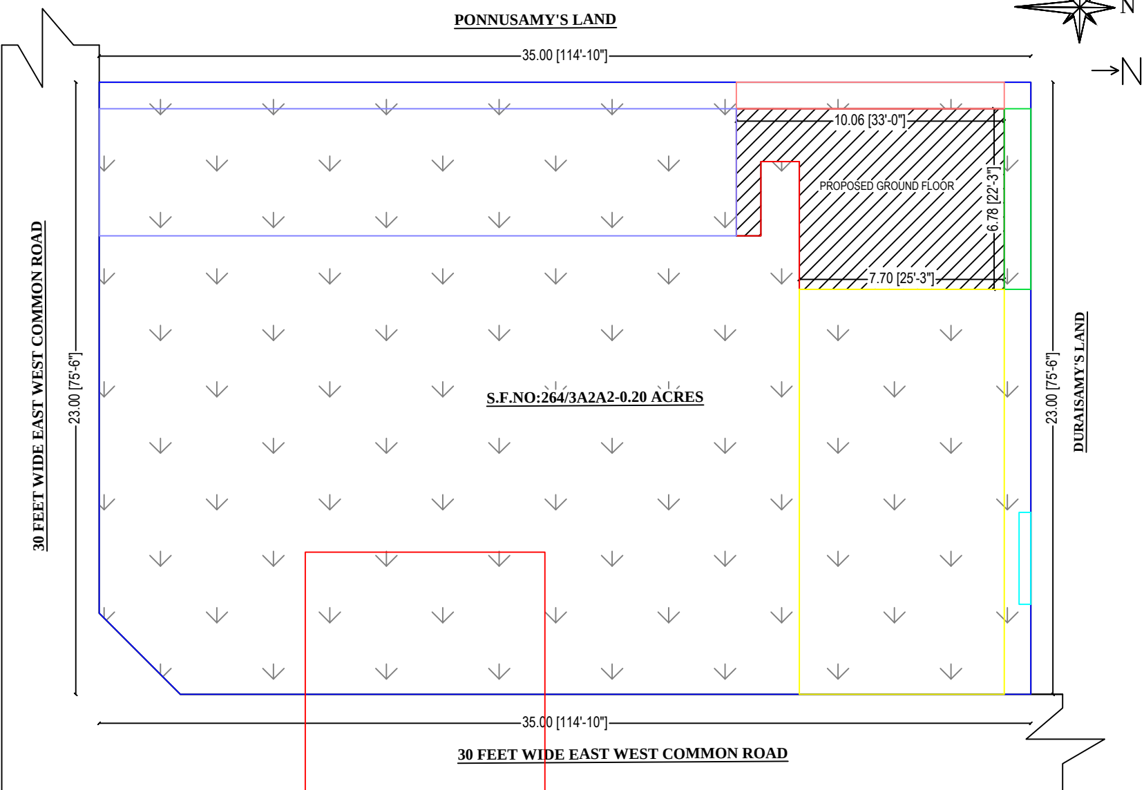
SITE PLAN
