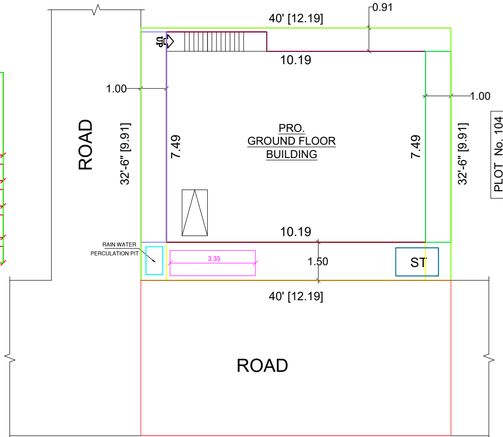
SITE PLAN
