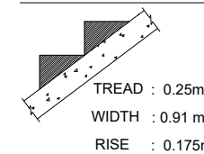
STAIRCASE DETAIL:
