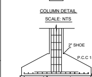
COLUMN DETAIL SCALE: NTS
