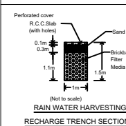
RAIN WATER HARVESTING RECHARGE TRENCH SECTION
