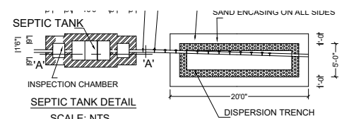
SEPTIC TANK DETAIL SCALE: NTS
