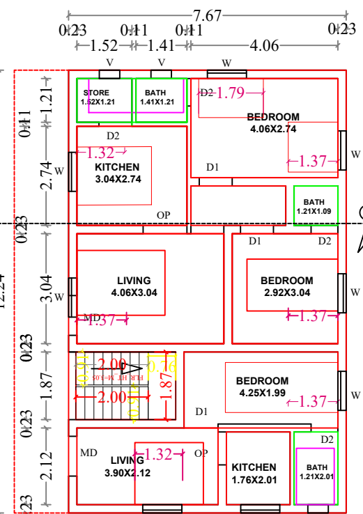
PROPOSED SECOND FLOOR
