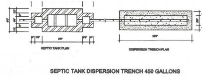
SEPTIC TANK DISPERSION TRENCH 450 GALLONS
