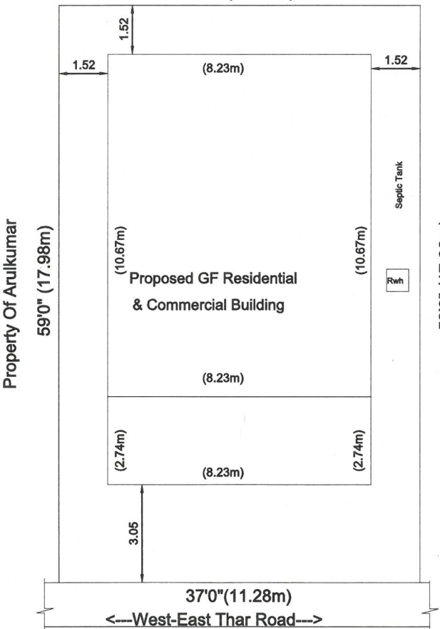
SITE PLAN
