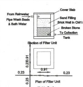
Section of Filter Unit
