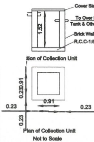
Plan of Collection Unit
