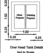
Over Head Tank Details
