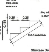
Staircase Detail
