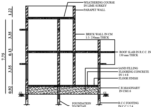
East Side Section On "AB"
