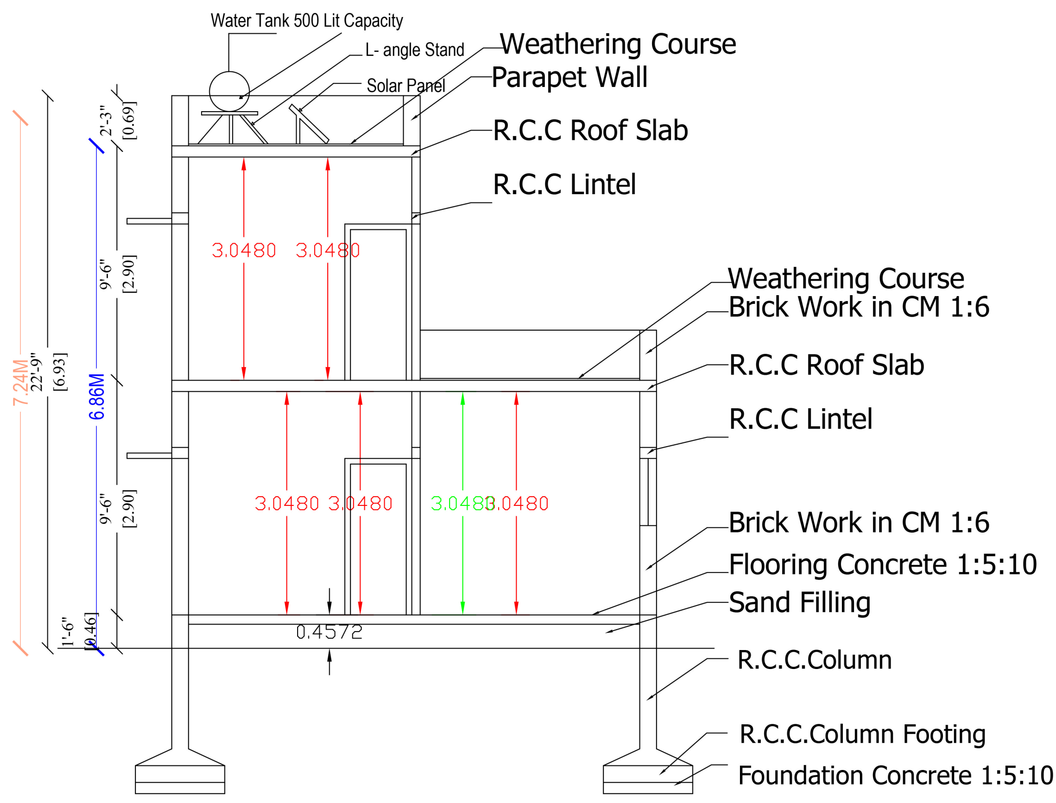
SECTION-AA
