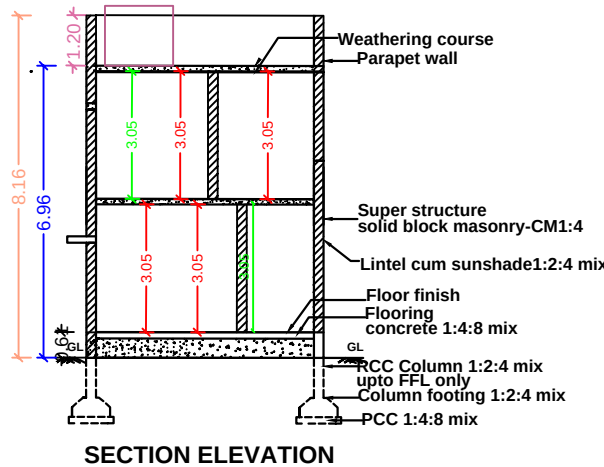
SECTION ELEVATION
