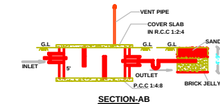
SECTION-AB
