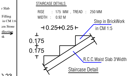
STAIRCASE DETAILS
