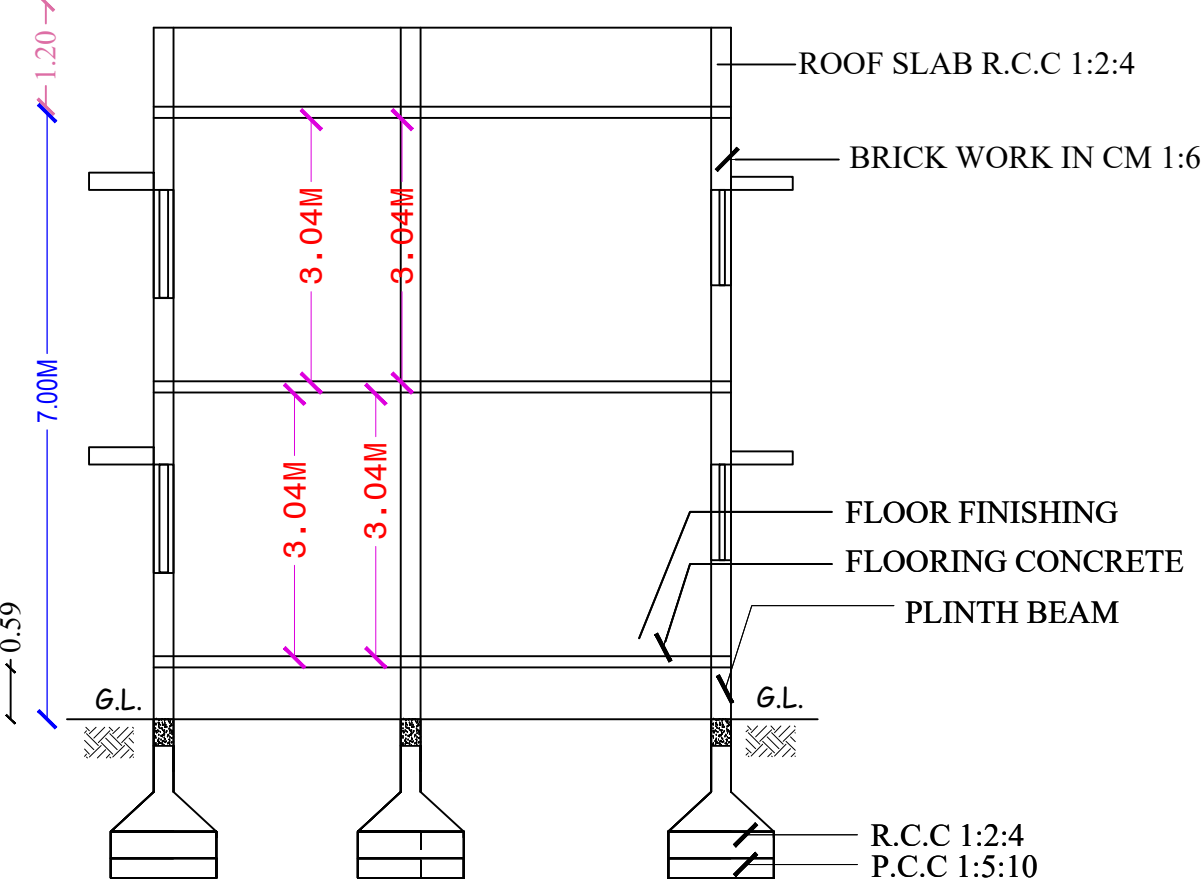
SECTION "A-A"
