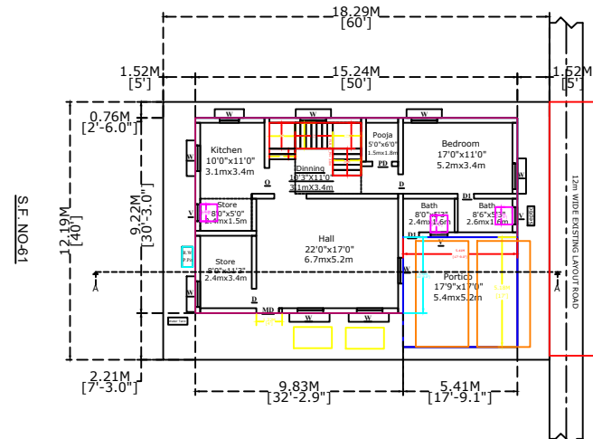
Site Cum Ground Floor Plan
