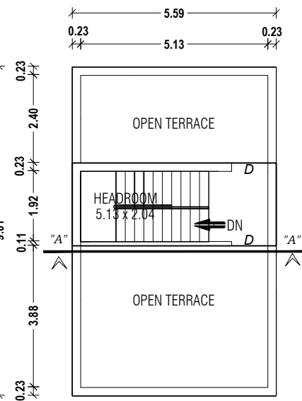
PRO. TERRACE FLOOR PLAN
