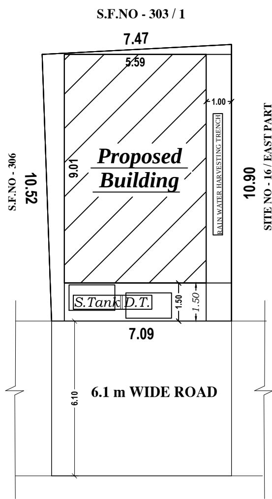
SITE PLAN
