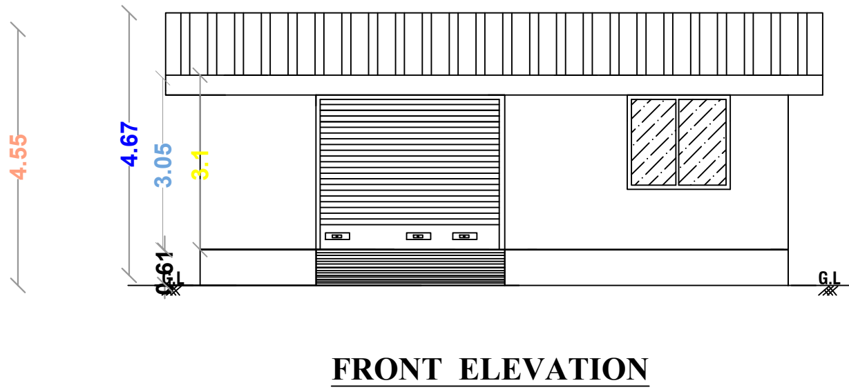
FRONT ELEVATION
