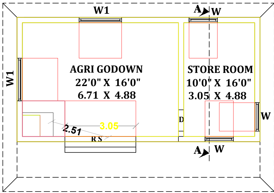
AGRI GODOWN PLAN
