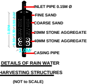
SECTION-AB
