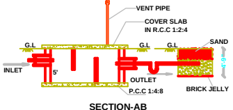
SECTION-AB
