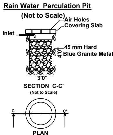
Rain Water Perculation Pit (Not to Scale)
