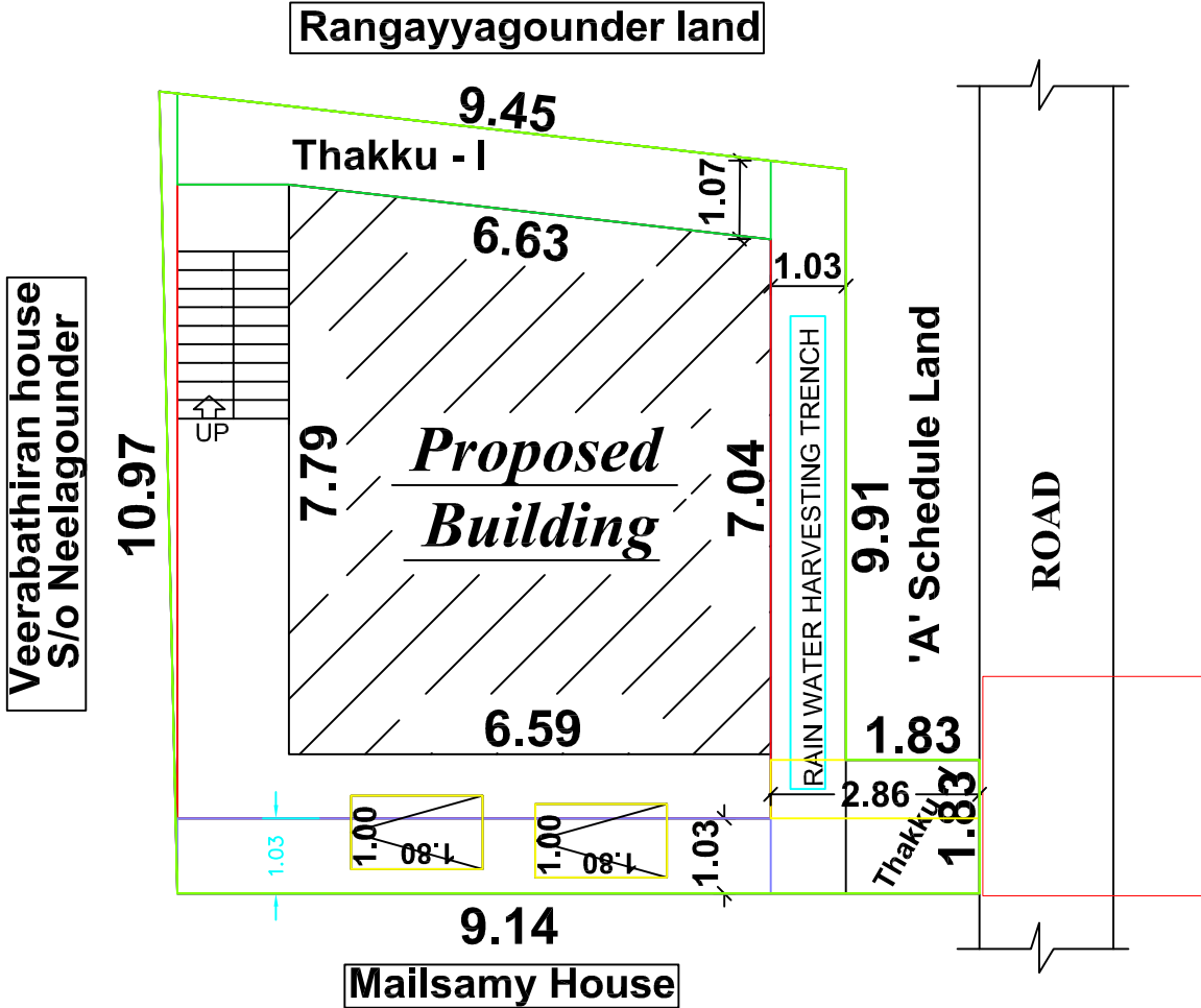
SITE PLAN
