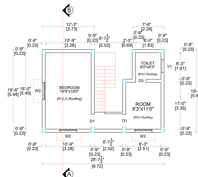
PROPOSED FIRST FLOOR PLAN (RCC ROOF)
