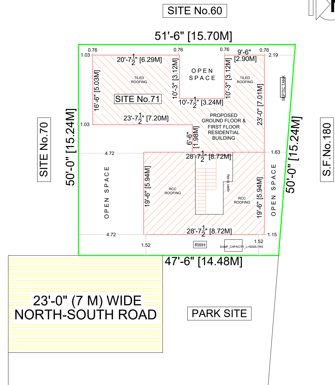
SITE PLAN
