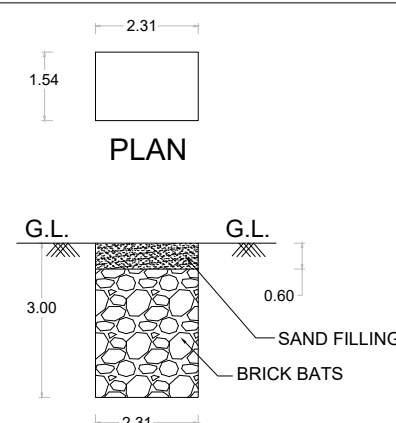
SECTION Not to Scale
