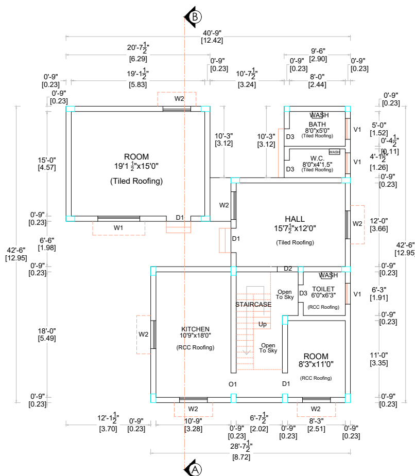
PROPOSED GROUND FLOOR PLAN (RCC ROOF AND TILES ROOF)
